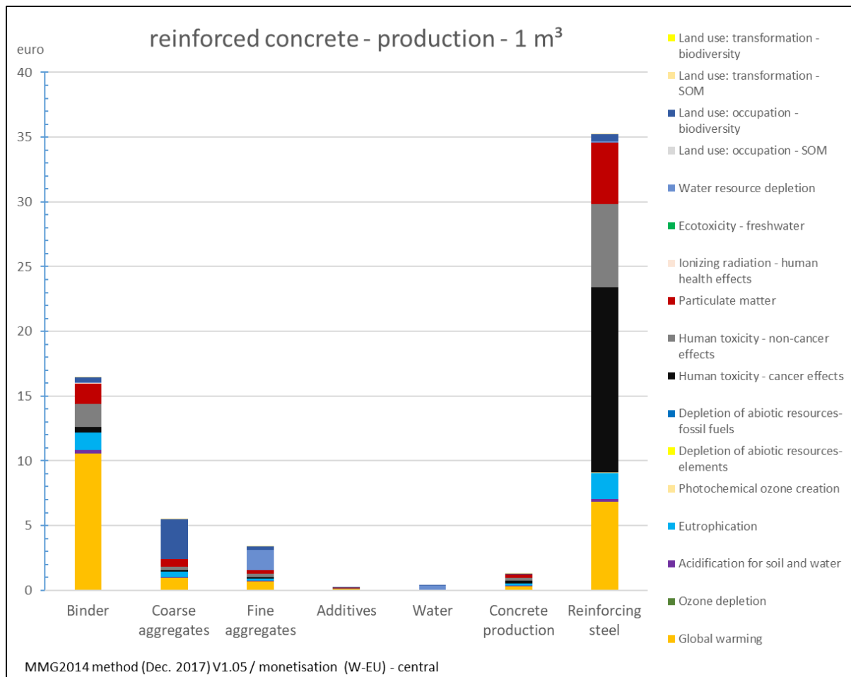
Figure 23: Environmental impact of the production of 1m 3 of reinforced concrete for road pavements (modules A1-A3), per component and per indicator.
