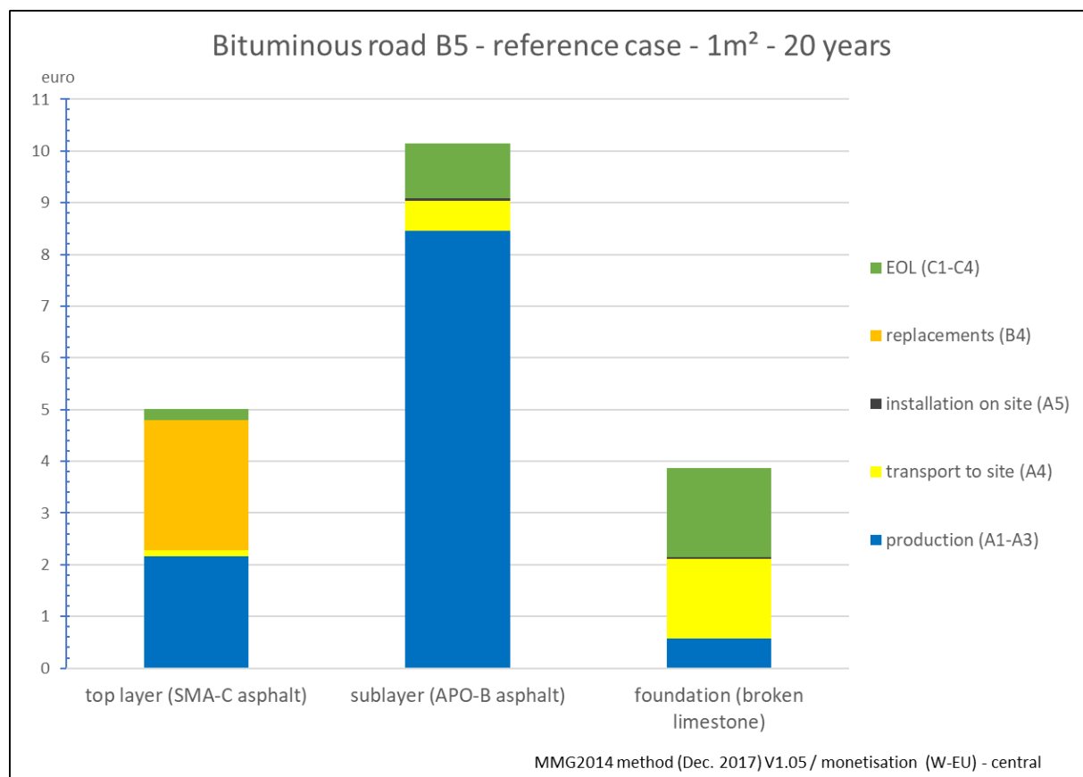
Figure 6: Environmental impact of 1m 2 of the reference bituminous road over 20 years, per layer and per lifecycle phase.
