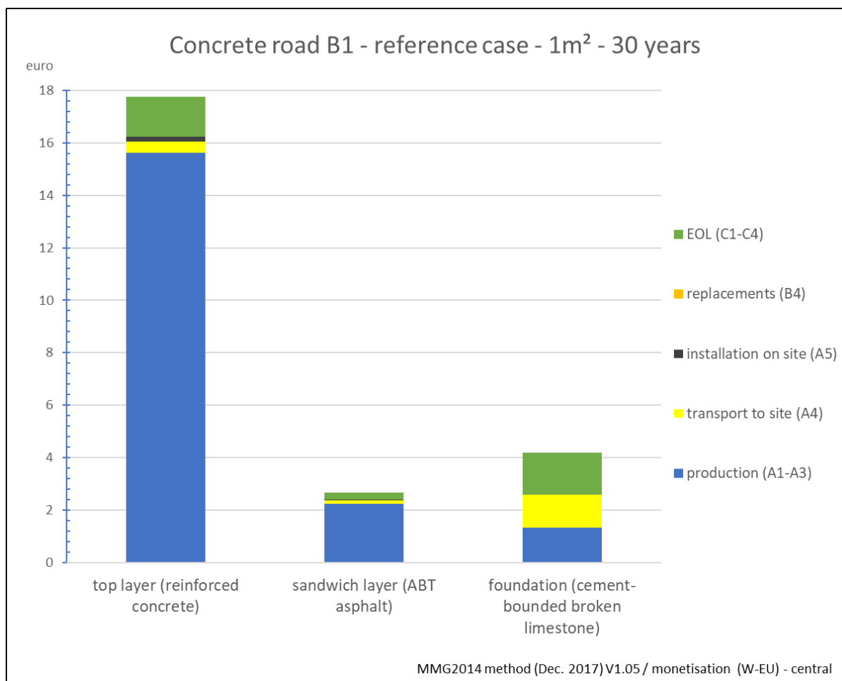
Figure 10: Environmental impact of 1 m 2 of the reference concrete road over 30 years, per layer and per lifecycle phase.
