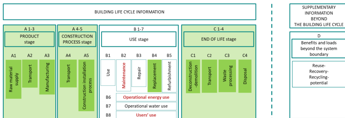
Figure 4: Indication (in green) of the different life cycle stages considered for the LCA study of road variants (according to the modules specified in EN 15978 [3] and prEN 17472 [2]). The life cycle stages indicated in red are different from the current TOTEM methodology for buildings and are not considered in this study.
